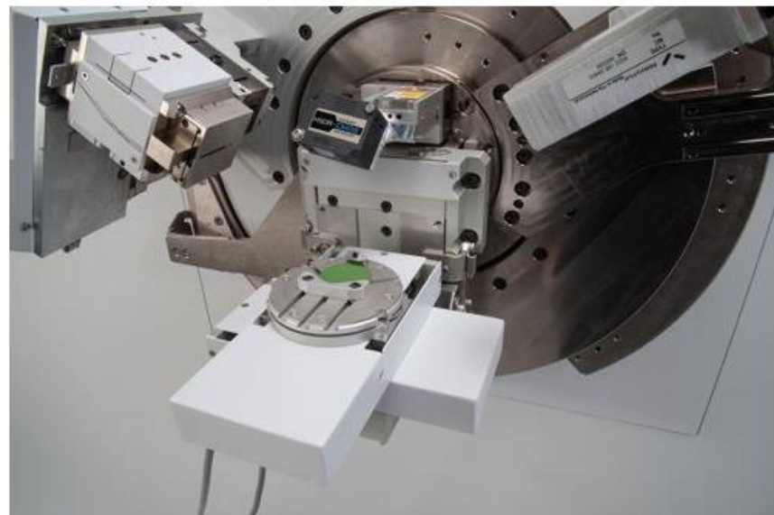
Height Sensor Mounted
